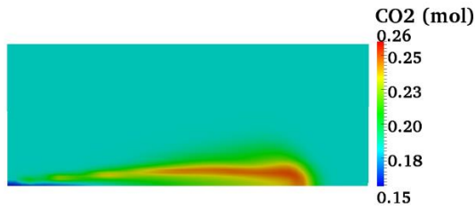
Figure 15: Carbone Dioxide distribution in the cylinder
